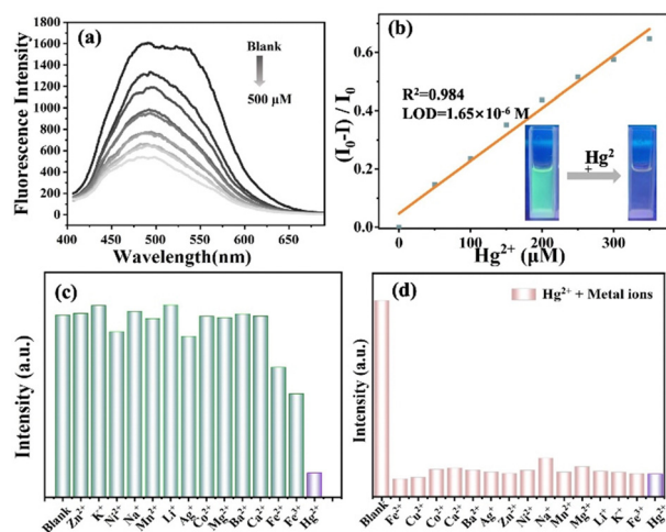
Fig. 2 (a) The fluorescence emission spectrum of DvDf-C3XJ-COF dispersed in EtOH:H 2 O = 1:1 with the addition of different amounts of Hg 2+ (0 to 500 \mu M). (b) The linear relationship between the fluorescence intensity of DvDf-C3XJ-COF with the concentration of Hg 2+ (Inset: A photograph demonstrating the fluorescence change of DvDf-C3XJ-COF in EtOH:H 2 O = 1:1 following the addition of 300 \mu M Hg 2+ , illuminated under a UV lamp with \lambda_{\text{ex}} = 365 nm). (c) The fluorescence intensity ratio of DvDf-C3XJ-COF in the presence of different metal ions (300 \mu M). (d) The fluorescence intensity ratio of DvDf-C3XJ-COF + Hg 2+ in the presence of different metal ions (300 \mu M).
