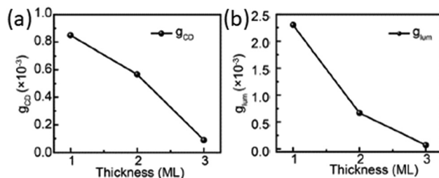
Fig. 29 (a) g_{\text{CD}} and (b) g_{\text{CPL}} of (S/R\text{-MPA})_2\text{Cs}_{n-1}\text{Pb}_n\text{Br}_{3n+1} as a function of the layer thickness \langle n \rangle . Reprinted with permission from ref. 49 Copyright©2023 Wiley-VCH GmbH.
