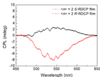
Fig. 27 CPL spectra of (R/S\text{-}Rac\text{-MBA})_2(\text{CsMA})\text{Pb}_2\text{Br}_7 . Reprinted with permission from ref. 47 Copyright©2022 American Chemical Society.
