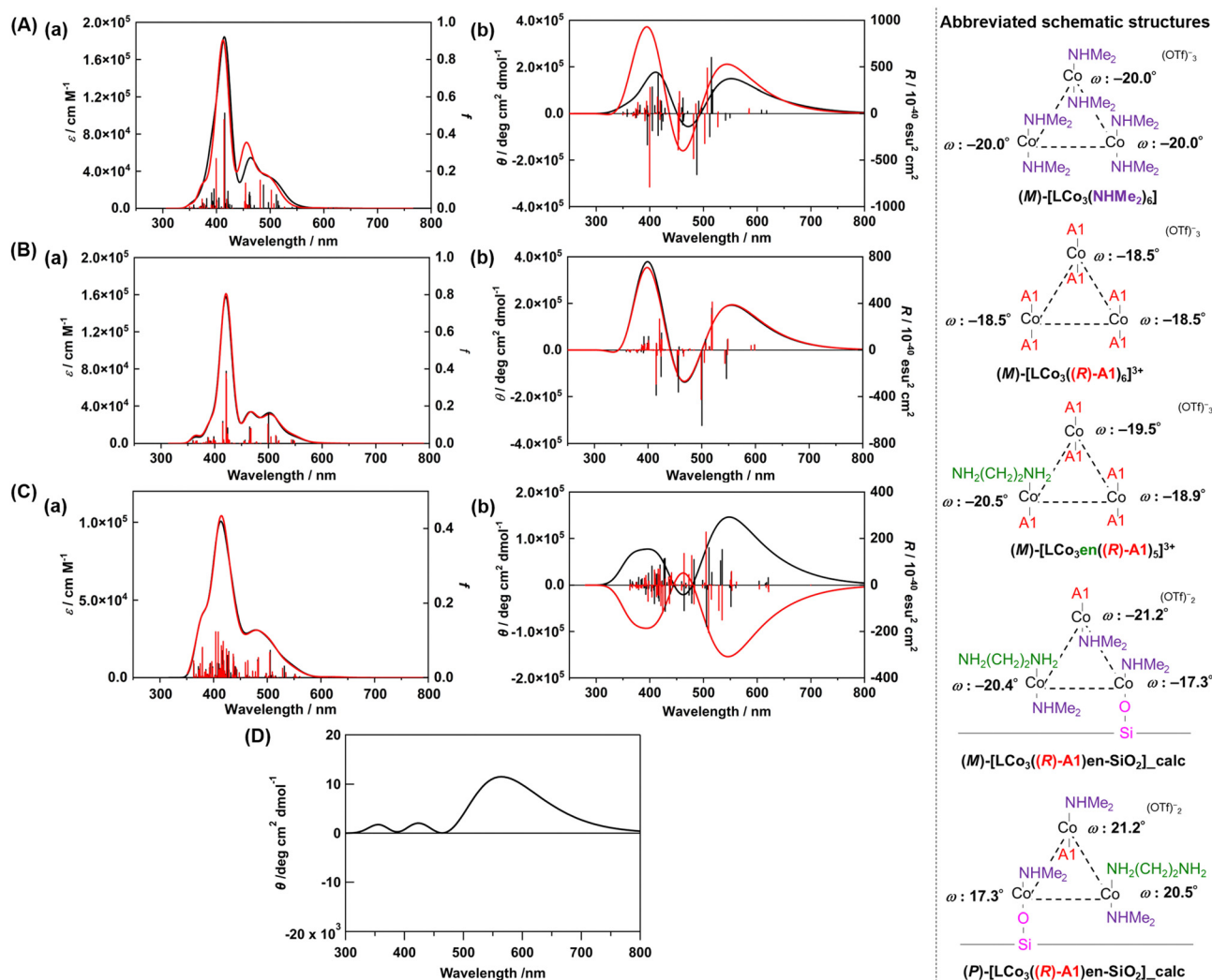
Fig. 2 (A) Calculated (a) UV-vis and (b) CD spectra of (M) -[ \text{LCo}_3(\text{NHMe}_2)_6 ] ^{3+} (black) and (M) -[ \text{LCo}_3((R)\text{-A1})_6 ] ^{3+} (red) (in acetonitrile). (B) Calculated (a) UV-vis and (b) CD spectra of (M) -[ \text{LCo}_3((R)\text{-A1})_6 ] ^{3+} (black) and (M) -[ \text{LCo}_3\text{en}((R)\text{-A1})_5 ] ^{3+} (red) (in vacuum). (C) Calculated (a) UV-vis and (b) CD spectra of the modelled structure of \text{LCo}_3((R)\text{-A1})/\text{en-SiO}_2\text{_{calc}} ( M configuration) (black) and \text{LCo}_3((R)\text{-A1})/\text{en-SiO}_2\text{_{calc}} ( P configuration) (red) (in vacuum). (D) The summed simulated CD spectrum of the modelled structure of \text{LCo}_3((R)\text{-A1})/\text{en-SiO}_2\text{_{calc}} ( M configuration) and \text{LCo}_3((R)\text{-A1})/\text{en-SiO}_2\text{_{calc}} ( P configuration) with the ratio of 55/45. Abbreviated schematic structures (see ESI ^\dagger and Fig. S2 for details) of the optimized trinuclear cobalt complexes are also presented. The torsion angles of each saloph moiety of the optimized structures under vacuum are also shown as \omega .
