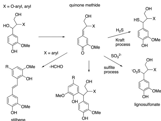
Fig. 10 Structures of condensed units found in Kraft lignin and liginosulfonate, formed from \beta -aryl ether units ( \text{X} = \text{O-aryl} ) and diarylpropane units ( \text{X} = \text{aryl} ).
