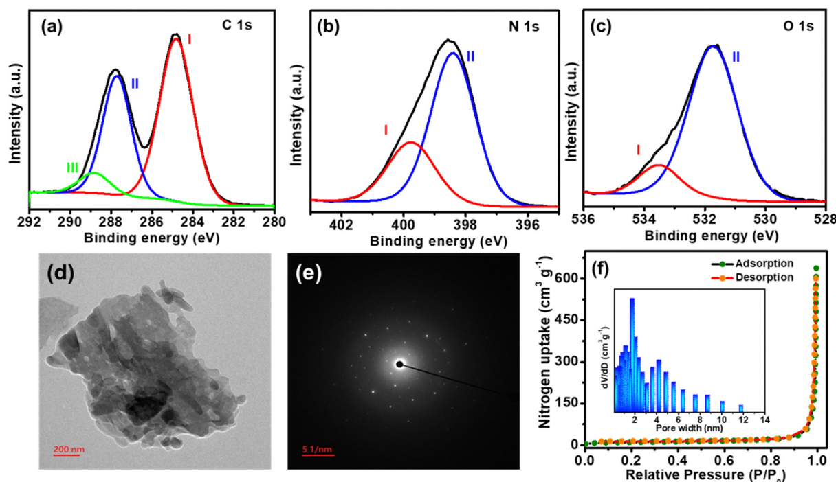
Fig. 1 Core level XPS spectra for (a) C 1s, (b) N 1s, and (c) O 1s of TP-COF. (d) TEM images and (e) corresponding SEAD image of TP-COF. (f) \text{N}_2 adsorption-desorption analysis of TP-COF and the corresponding pore size distribution plot of TP-COF in the inset.
