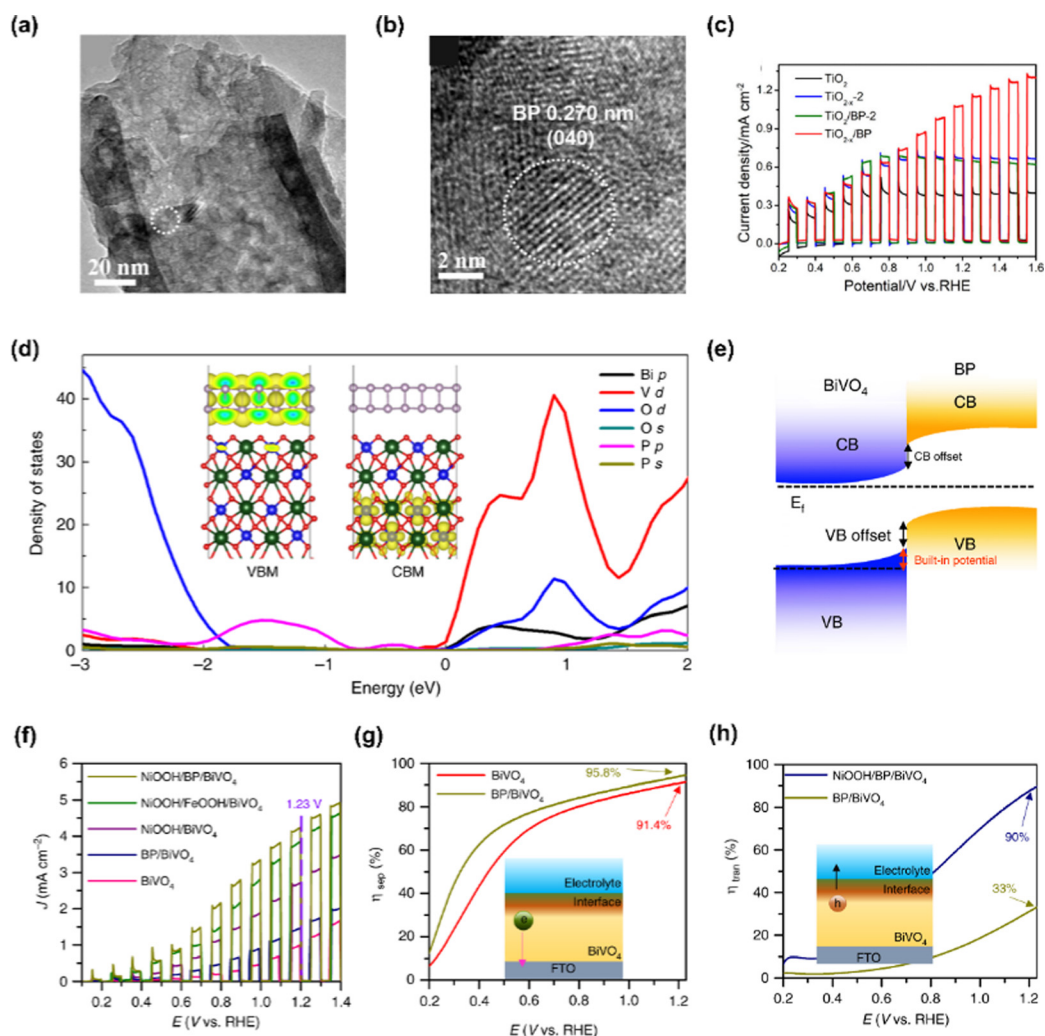
Fig. 8 (a) TEM and (b) HR-TEM images of \text{TiO}_2\text{-x/BP} . (c) LSV curves of \text{TiO}_2 , \text{TiO}_2\text{-x-2} , \text{TiO}_2\text{/BP-2} , and \text{TiO}_2\text{-x/BP} . Copyright 2020, American Chemical Society. (d) Density of states (DOS) of \text{BP/BiVO}_4 heterojunction. (e) Energy band diagram of \text{BP/BiVO}_4 . (f) Chopped LSV curves of \text{BiVO}_4 , \text{BP/BiVO}_4 , \text{NiOOH/BiVO}_4 , \text{NiOOH/FeOOH/BiVO}_4 , and \text{NiOOH/BP/BiVO}_4 . (g) Charge separation efficiencies and (h) charge transfer efficiencies of \text{BiVO}_4 and \text{BP/BiVO}_4 . Copyright 2019, Springer Nature.
