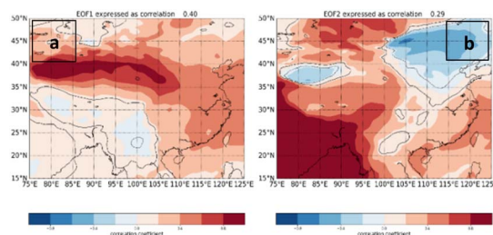
Fig. 9 The loading of empirical orthogonal function (EOF) of average dust surface mass concentration of \text{PM}_{2.5} during the winter season (from November to February) from 1980 to 2018 across China: (a) EOF1 and (b) EOF2.
