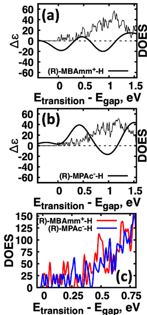
Fig. 5 Comparison of chirality transfer for ( R )-MBAm + -H and ( R )-MPAc - -H. Overlay of CD spectra and DOES for (a) ( R )-MBAm + -H and (b) ( R )-MPAc - -H. (c) DOES overlaid for ( R )-MBAm + -H (red) and ( R )-MPAc - -H (blue).
