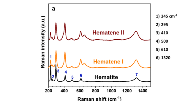
Fig. 3 (a) Representative Raman spectra of bulk Hematite and exfoliated Hematene nanoplatelets. Analysis of T mode (peak 1) at bulk hematite (b), Hematene II (c) and Hematene I (d).
