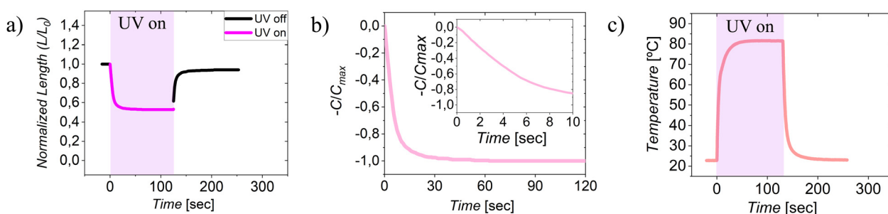
Fig. 4 Photomechanical response in air at RT of a uniaxial oriented sample (70 \mu\text{m} thick) with the director along its long axis. A metal weight of 1 g is attached to the lower extreme of the sample. (a) Normalized length ( L/L_0 ) of the LC elastomer during UV irradiation (purple line) in air using two UV LEDs irradiating each face of the sample with an intensity of 90 mW cm -2 and subsequent partial recovery of the length when UV illumination ceases (black line). (b) Normalized contraction expressed in negative values ( -C/C_{max} ) during exposure to UV light. Normalized contraction is given in negative values to show the dynamic as a decay. (b inset) Detail of the normalized contraction, in negative values, during the first 10 seconds of UV light irradiation. (c) Temporal dependence of the temperature of the LCE surface during UV light irradiation (purple square) and after switching off the UV illumination.
