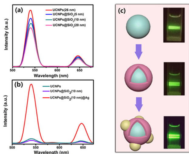
Fig. 11 (a) UC emission spectra of pure UCNP and UCNP@SiO 2 core/shell NPs. (b) UC emission spectra of the UCNP, UCNP@SiO 2 (10 nm) NPs and UCNP@SiO 2 (10 nm)@Ag NPs. (c) Schematic illustrations of these three types of NPs and their digital luminescence photos. 81
