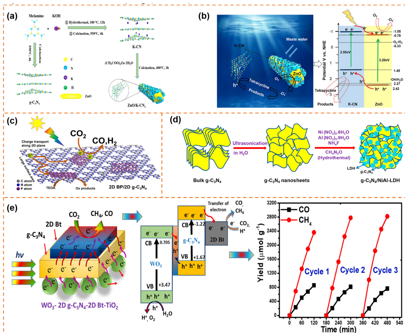
Fig. 12 (a) Schematic diagram of the synthesis and assembly route of photocatalyst materials. (b) Schematic diagram of the charge separation and photocatalytic mechanism of type-II ZnO/K-CN heterojunctions under simulated sunlight. Reprinted with permission from ref. 166, © American Chemical Society 2020. (c) Illustration of the photocatalytic mechanism of the 2D BP/2D g\text{-C}_3\text{N}_4 system under visible-light irradiation. Reprinted with permission from ref. 169, © Elsevier B.V. 2020. (d) Schematic illustration of the synthesis process of g\text{-C}_3\text{N}_4/\text{NiAl-LDH} hybrid heterojunctions. Reprinted with permission from ref. 170, © American Chemical Society 2018. (e) Proposed mechanism and stability analysis of photocatalytic \text{CO}_2 reduction with \text{H}_2\text{O} over the Bt-mediated \text{WO}_3/g\text{-C}_3\text{N}_4 composite under visible-light irradiation. Reprinted with permission from ref. 172, © American Chemical Society 2020.
