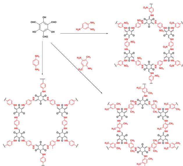
Fig. 4 Synthesis of three COFs with identical principal skeletons (TPA-COF-X, where X = H, (\text{CH}_3)_2 , or \text{NO}_2 ).
