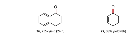
Fig. 4 Photoanode-mediated C–H oxygenation at the \alpha -position of the alkane and arene.
