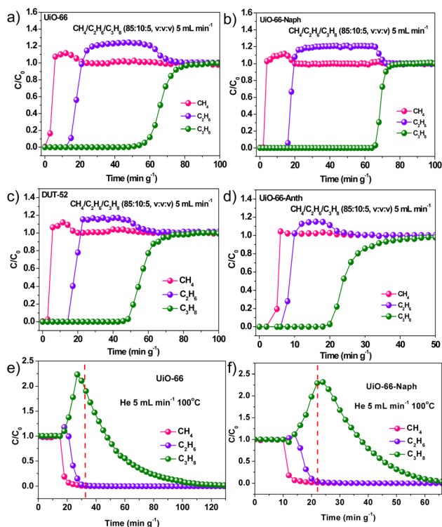
Fig. 5 Transient breakthrough curves (a–d) of \text{CH}_4/\text{C}_2\text{H}_6/\text{C}_3\text{H}_8 (85 : 10 : 5, v/v/v) mixture for UiO-66, UiO-66-Naph, DUT-52 and UiO-66-Anth, and desorption curves (e and f) for UiO-66 and UiO-66-Naph, respectively.
