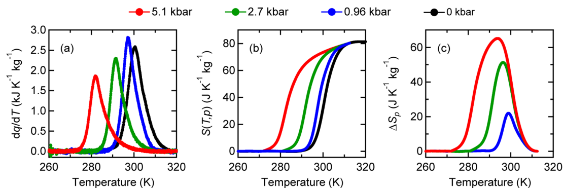
Fig. 2 (a) Heat flow curves divided by the cooling rate \text{dq/dT} , (b) corresponding entropy as a function of temperature, and (c) isothermal entropy changes of \text{NdCu}_3\text{Fe}_4\text{O}_{12} under various applied pressures.
