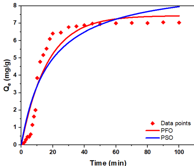
Fig. 8 Kinetic profiles at pH 7.5 and 23 °C for the coagulation-like removal of arsenic at pH 7.5 with both H_2AsO_4^- and HAsO_4^{2-} species present. The fitted lines correspond to the best-fit results for the PFO and PSO kinetic models.
