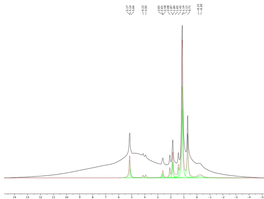
Fig. 10 ^1\text{H} MAS NMR and deconvoluted spectra of pure sHAP (2Q: 15 \mu\text{L g}^{-1} Neutrase, 7.5 \mu\text{L g}^{-1} Lipozyme CALB L, 6 h, 40 ^\circ\text{C} ).
