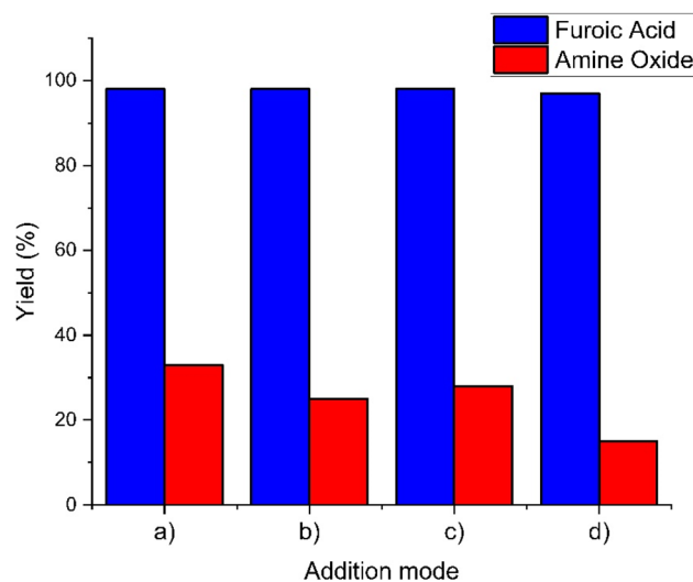
Fig. 3 Effect of the addition mode of hydrogen peroxide on the yield of furoic acid and amine oxide. (a) Addition of hydrogen peroxide into a premixed mixture of furfural and amine at 55 °C, (b) addition of hydrogen peroxide (1.3 eq.) and amine into furfural at 55 °C through 10 additions, (c) addition of hydrogen peroxide (1.3 eq.) and furfural into amine at 55 °C through 10 additions, and (d) addition of hydrogen peroxide into a premixed amine-furfural mixture at 55 °C (addition of the first 0.5 eq. over 10 h).
