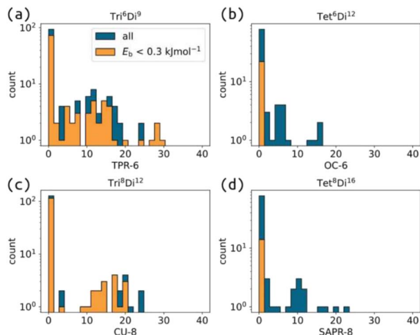
Fig. 6 Distribution of the deviation from the ideal shapes for (a) \text{Tri}^6\text{Di}^9 (shape measure: TPR-6), (b) \text{Tet}^6\text{Di}^{12} (shape measure: OC-6), (c) \text{Tri}^8\text{Di}^{12} (shape measure: CU-8) and (d) \text{Tet}^8\text{Di}^{16} (shape measure: SAPR-8) with torsion-restrictions for tritopic or tetratopic building blocks. Blue distributions are all cages, and orange is for stable cages. This data is on a log scale due to the high proportion of cages near zero.
