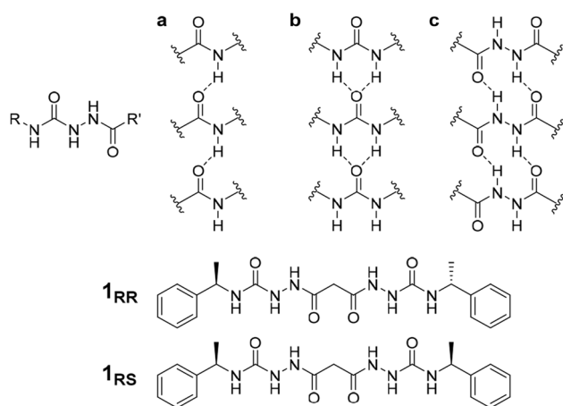
Fig. 1 Structure of the acyl-semicarbazide group and target compounds of type 1 along with gel-promoting synthons by acyl-semicarbazides. (a) C(4) motifs between amides. (b) R 2 2 (6) α-tapes between urea groups. (c) R 3 2 (10) motifs in hydrazide-based gelators.
