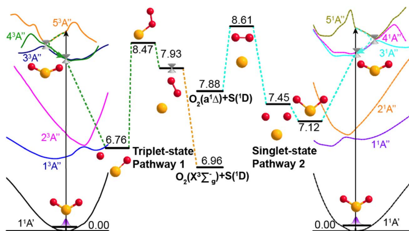
Fig. 4 Dissociation pathways of \text{SO}_2 leading to \text{O}_2(\text{X}^3\Sigma_g^-) + \text{S}(^1\text{D}) products via the triplet state manifold (left) and to \text{O}_2(\text{a}^1\Delta_g) + \text{S}(^1\text{D}) products via the singlet state manifold. The schematics of the simplified PECs for the ground and the first five excited states of ^3\text{A}'' symmetry (left) and the first five states of ^1\text{A}'' symmetry (right) support different paths leading to \text{S} + \text{O}_2 product formation. Dashed arrows indicate possible non-adiabatic pathways and the geometries and energies (in eV) of key intermediate structures along the dissociation pathways are also indicated. The horizontal axis represents the reaction coordinate, and the vertical axis is the potential energy (in eV).
