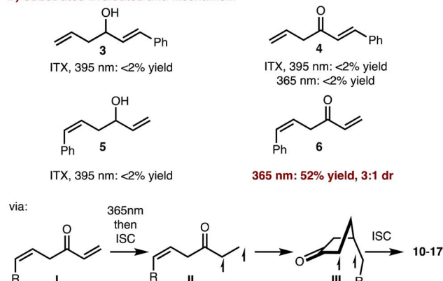
Scheme 1 Crossed [2 + 2]-cycloaddition.
