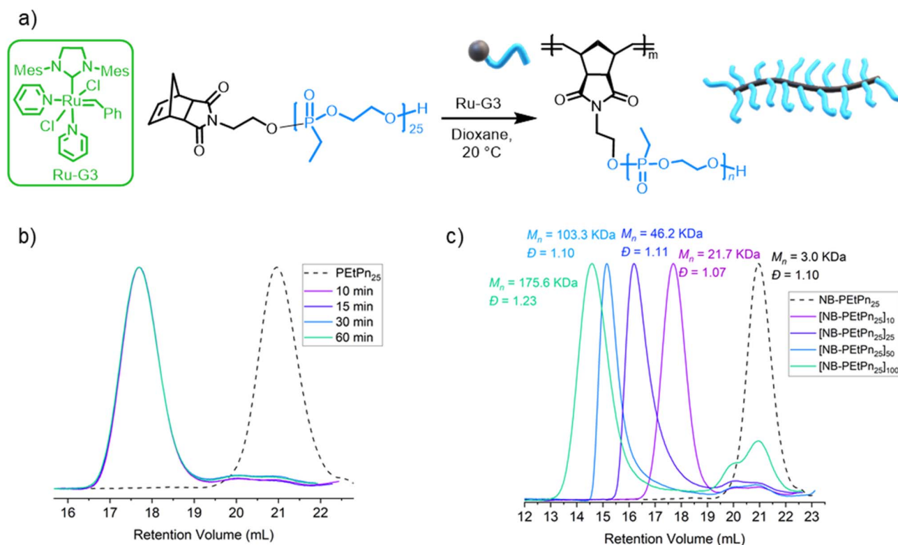
Fig. 2 (a) Synthetic scheme of the graft-through ROP of 3 using the Grubbs 3 rd -generation complex (Ru-G3). (b) SEC elugrams (2 mg mL -1 ) (normalized RI) at different reaction times for the polymerization of ROP of norbornene-based PETn 25 using the Ru-G3 catalyst with varying PETn 25 : Ru-G3 ratios of 10 : 1 (measured in DMF (0.1 M LiCl) at 60 °C vs. polystyrene standards using the RI detector by SEC). (c) SEC elugrams (2 mg mL -1 ) (normalized RI) of polymers from ROP of norbornene-based PETn 25 using the Ru-G3 catalyst with varying PETn 25 : Ru-G3 ratios (10, 25, 50 and 100) (measured in DMF (0.1 M LiCl) at 60 °C vs. polystyrene standards using the RI detector by SEC).
