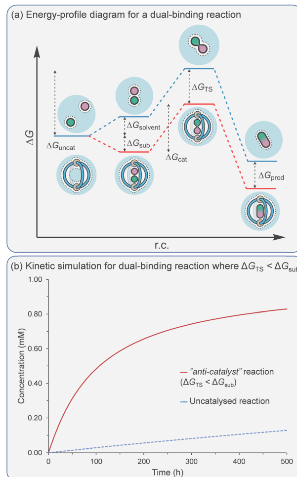
Fig. 8 (a) Energy profile diagram for a cage-mediated dual-binding reaction. (b) Kinetic simulation of a dual binding reaction where the stabilisation of the substrates, \Delta G_{\text{sub}} , is greater than stabilisation of the TS, \Delta G_{\text{TS}} . Simulation conditions: [\text{subA}]_0 = [\text{subB}]_0 = [\text{cage}]_0 = 1 \text{ mM} ; k_{\text{subA-on}} = k_{\text{subB-on}} = 1.0 \times 10^{11} \text{ M}^{-1} \text{ s}^{-1} ; k_{\text{subA-off}} = k_{\text{subB-off}} = 1.0 \times 10^6 \text{ s}^{-1} ; K_{\text{TS}} = 3.3 \times 10^8 \text{ M}^{-1} ; K_{\text{prod}} = 0 \text{ M}^{-1} ; k_{\text{uncat}} = 0.30 \text{ M}^{-1} \text{ s}^{-1} ( \Delta G_{\text{uncat}} = 23 \text{ kcal mol}^{-1} ); k_{\text{cat}} = 0.01 \text{ s}^{-1} ( \Delta G_{\text{uncat}} = 25 \text{ kcal mol}^{-1} ).
