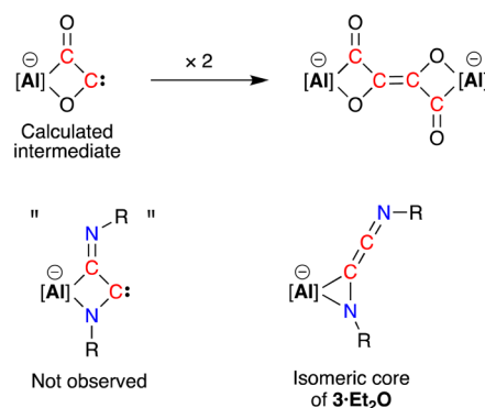
Fig. 6 Calculated carbene intermediate in the formation of the [(\text{CO})_4]^{4-} ligand, with the analogous dimerised isocyanide (not observed) and isomeric core of 3 ·Et 2 O.
