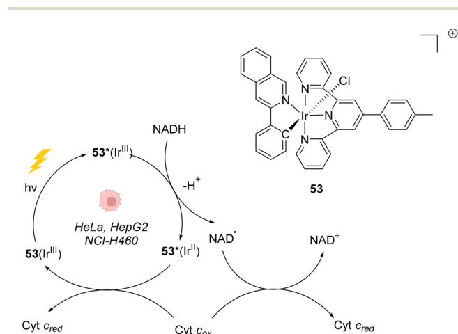
Fig. 21 Photoredox Ir III -based catalytic cycle proposed by Sadler et al. for in cellulo light-induced NADH oxidation under hypoxic conditions. 61
