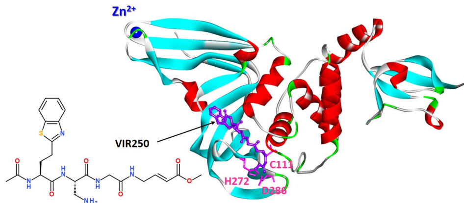
Fig. 20 X-ray structure of PLpro in complex with covalent peptide inhibitor VIR250 (PDB: 6WUU).
