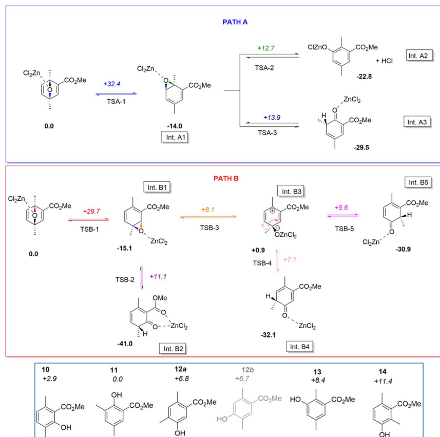
Scheme 1 Top: DFT proposed reaction paths for the aromatization of the Diels–Alder adduct formed by the reaction of dimethylfuran on methylpropiolate in presence of ZnCl 2 . The structures of the reagent, intermediates and products are displayed. Bottom: Structure and relative energies (E+ZPE) of all considered phenolic products. Relative energies (E+ZPE) are given in kcal mol -1 (as computed at the M062X/6-311++G(d,p) level of theory). Phenol 12b is coloured in gray to remind that no reaction route was found to lead to this product.
