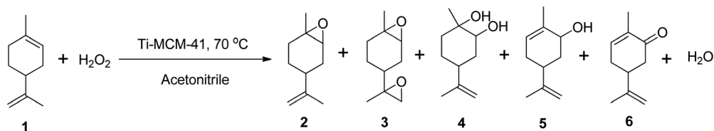
Scheme 11 Epoxidation of (1) (R) -(+)-limonene with \text{Ti-MCM-41} producing (2) limonene-1,2-epoxide, (3) limonene bis-epoxide, (4) limonene-1,2-diol, (5) carveol and (6) carvone.
