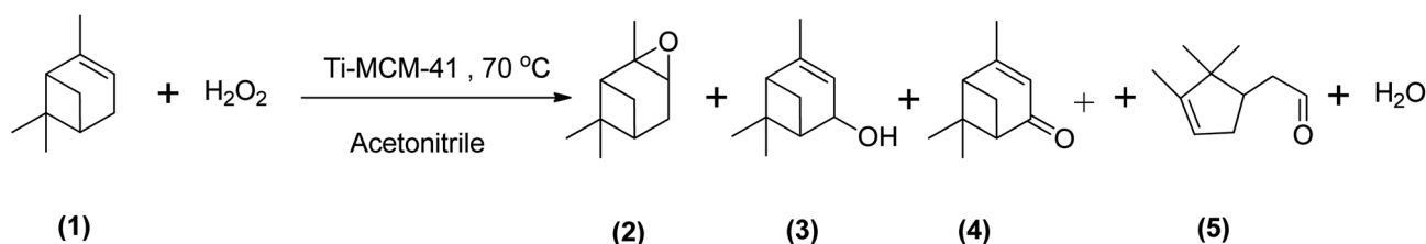
Scheme 12 Epoxidation of (1) \alpha -pinene with \text{Ti-MCM-41} catalyst producing (2) \alpha -pinene oxide, (3) verbenol, (4) verbenone and (5) campholenic aldehyde.
