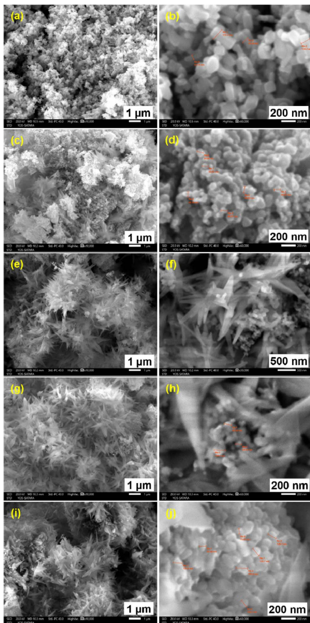
Fig. 7 FESEM images of ZnO (a and b), 5% AlCl 3 @ZnO (c and d), 10% AlCl 3 @ZnO (e and f), 15% AlCl 3 @ZnO (g and h), 20% AlCl 3 @ZnO (i and j).
