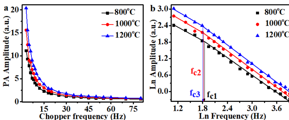
Fig. 7 (a) Comparison of PA signal with frequency at 160 mW excitation power for samples annealed at 800 °C, 1000 °C, and 1200 °C (b) In–ln plot between PA signal and frequency to show variation in critical frequency.
