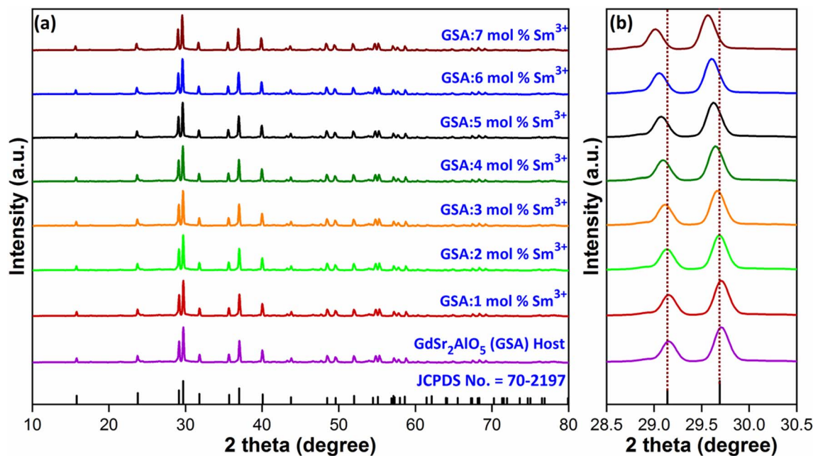
Fig. 2 (a) Diffraction profiles of \text{GdSr}_2\text{AlO}_5 and \text{Gd}_{1-x}\text{Sr}_x\text{AlO}_5:x\text{Sm}^{3+} ( x = 1-7 \text{ mol\% Sm}^{3+} ) phosphors (b) enlarged view of respective diffraction patterns.
