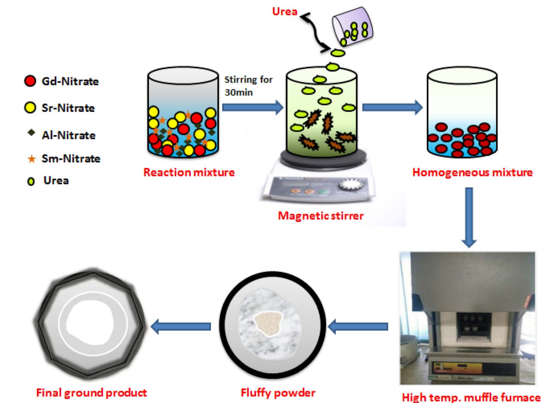
Fig. 1 Schematic diagram of GC method for the synthesis of \text{Gd}_{1-x}\text{Sr}_x\text{AlO}_5:x\text{Sm}^{3+} ( x = 1-7 \text{ mol\% Sm}^{3+} ) nanopowders.
