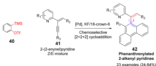
Scheme 7 Palladium-catalyzed selective [2 + 2 + 2] annulation.
