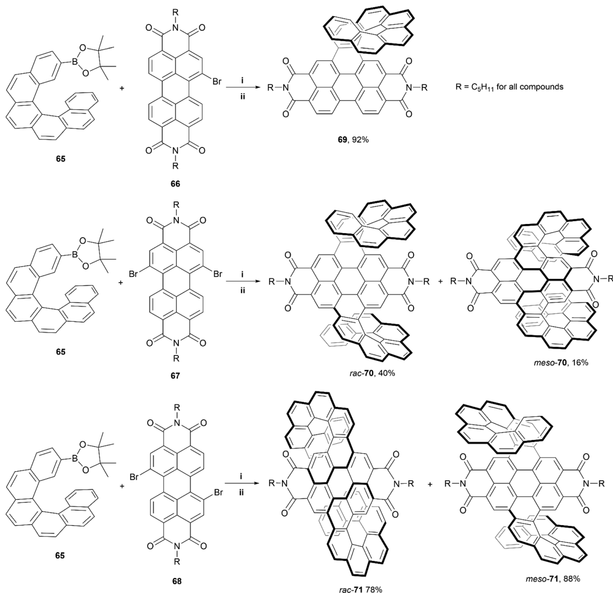
Scheme 13 Synthesis of PDI-helicene hybrid compounds; (i) 66 , 67 , or 68 (1.0 equiv.), 65 (1.2 equiv.), \text{Pd(dppf)Cl}_2 (0.1 equiv.), \text{K}_3\text{PO}_4 , THF, 90 °C; (ii) \text{I}_2 , h\nu , toluene, 100 °C. Note: Precyclized intermediates were separated via column chromatography prior to step ii.
