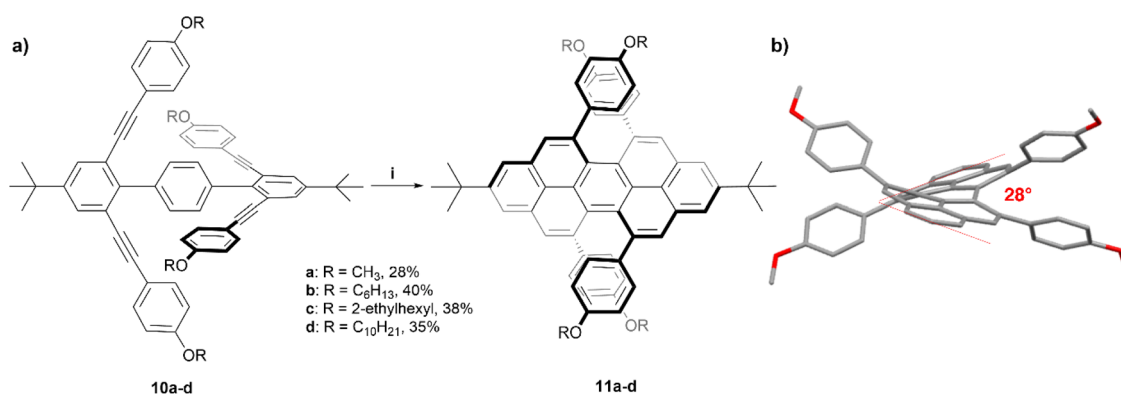
Scheme 2 (a) Synthesis of chiral peropyrene 11 ; (i) 10 (1.0 equiv.), TfOH (0.2 equiv.), DCM, -40^{\circ}\text{C} , 30 min; (b) published crystal structure of 11b showing twisting. Hydrogens and alkyl groups omitted for clarity.
