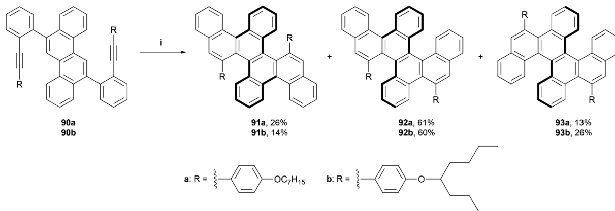
Scheme 18 Synthesis of double, triple and quadruple helices; (i) 90 (1.0 equiv.), DCM : TFA (98 : 2, v : v), 25 °C, 12 h.
