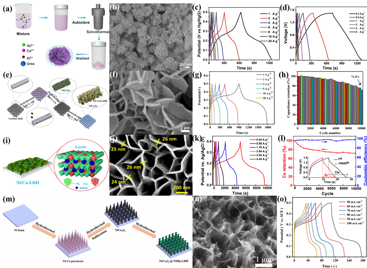
Fig. 5 (a) Schematic representation of the synthesis of NiCoAl LDH nanosheets, (b) SEM image of NiCoAl-LDH-9, (c) GCD curves of the NiCoAl-LDH-9 electrode at various current densities, (d) GCD curves of the device at different current densities. Adapted with permission from ref. 143 Copyright 2021, Elsevier B.V. (e) Schematic illustration of the synthesis processes of hierarchical NiCoAl-LDHs@NiCo 2 S 4 @CC, (f) SEM image of NiCoAl-LDHs@NiCo 2 S 4 @CC, (g) GCD curves of NiCoAl-LDHs@NiCo 2 S 4 @CC at various current densities, and (h) cycling stability performance of device at 1 A g -1 . Adapted with permission from ref. 145 Copyright 2021 Elsevier B.V. (i) Schematic diagram of the structural growth of NiCo LDHs on an NF substrate, (j) SEM image of NiCo LDHs, (k) GCD curves at different current densities, and (l) cycling stability and coulombic efficiency of the NiCo LDHs//AC with the inset showing the first and 10000th GCD curves. Adapted with permission from ref. 146 Copyright 2020, Elsevier Ltd. (m) Schematic illustration of the synthesis processes of NiCo 2 S 4 @NiMn-LDHs core-shell hybrid arrays on NF, (n) SEM image of NiCo 2 S 4 @NiMn-LDH, and (o) GCD curves at different current densities. Adapted with permission from ref. 147 Copyright 2021, Elsevier B.V.
