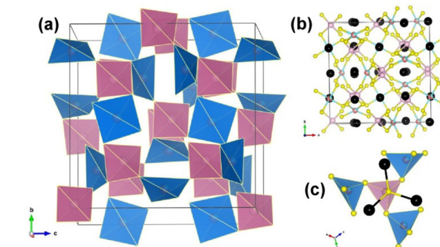
Fig. 13 Crystal structural of Ba 6 Cu 1.9 Mg 1.1 Sn 4 S 16 : (a) polyhedral packing model; (b) ball-and-stick model; (c) coordination environment of [(Cu/Mg)S 4 ] (pink) and [SnS 4 ] (blue) tetrahedra. Black: Ba; red: Mg; blue: Cu; pink: Sn; yellow: S. Copyright 2021 American Chemistry Society.
