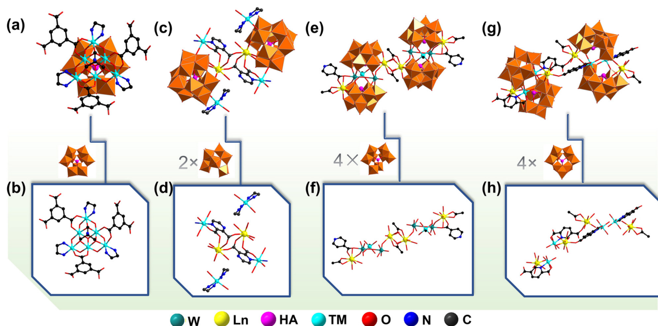
Fig. 1 Summary of representative structures of IOHPMs. (a and b) View of \{\text{Ni}_6(\text{Tris})(\text{en})_3(\text{BTC})_3(\text{B-}\alpha\text{-PW}_9\text{O}_{34})\} ( \text{Tris} = tris(hydroxymethyl)amino-methane, \text{en} = ethylenediamine) and its remaining part without \{\text{B-}\alpha\text{-PW}_9\text{O}_{34}\} . (c and d) View of \{[\text{Cu}(\text{en})_2][\text{Cu}(\text{PZDA})_2][(\alpha\text{-H}_2\text{SiW}_{11}\text{O}_{39})\text{Ce}(\text{H}_2\text{O})]\}_2^{6-} and its remaining part without \{\alpha\text{-H}_2\text{SiW}_{11}\text{O}_{39}\} . (e and f) View of \{[\text{Sn}(\text{CH}_3\text{W}_2\text{O}_4(\text{IN}))][(\text{B-}\alpha\text{-TeW}_8\text{O}_{31})\text{Ln}(\text{H}_2\text{O})(\text{CH}_3\text{COO})]\}_2^{20-} and its remaining part without \{\text{B-}\alpha\text{-TeW}_8\text{O}_{31}\} . (g and h) View of [\text{Ln}_2(\text{CH}_3\text{COO})_2(\text{H}_2\text{O})_4\text{Fe}_2(\text{HPDCA})_2(\text{B-}\beta\text{-TeW}_9\text{O}_{33})_2][\text{Ln}_2(\text{H}_2\text{O})_8\text{Fe}_2(\text{HPDCA})_2(\text{B-}\beta\text{-TeW}_9\text{O}_{33})_2]^{14-} and its remaining part without \{\text{B-}\beta\text{-TeW}_9\text{O}_{33}\} .
