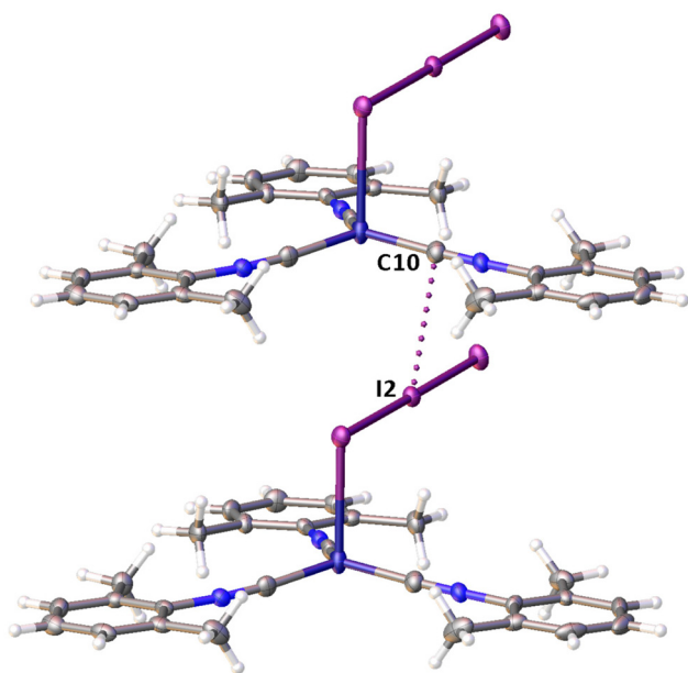
Fig. 4 The I...C contact in the structure of 2 \cdot \frac{1}{2}I_2 .
