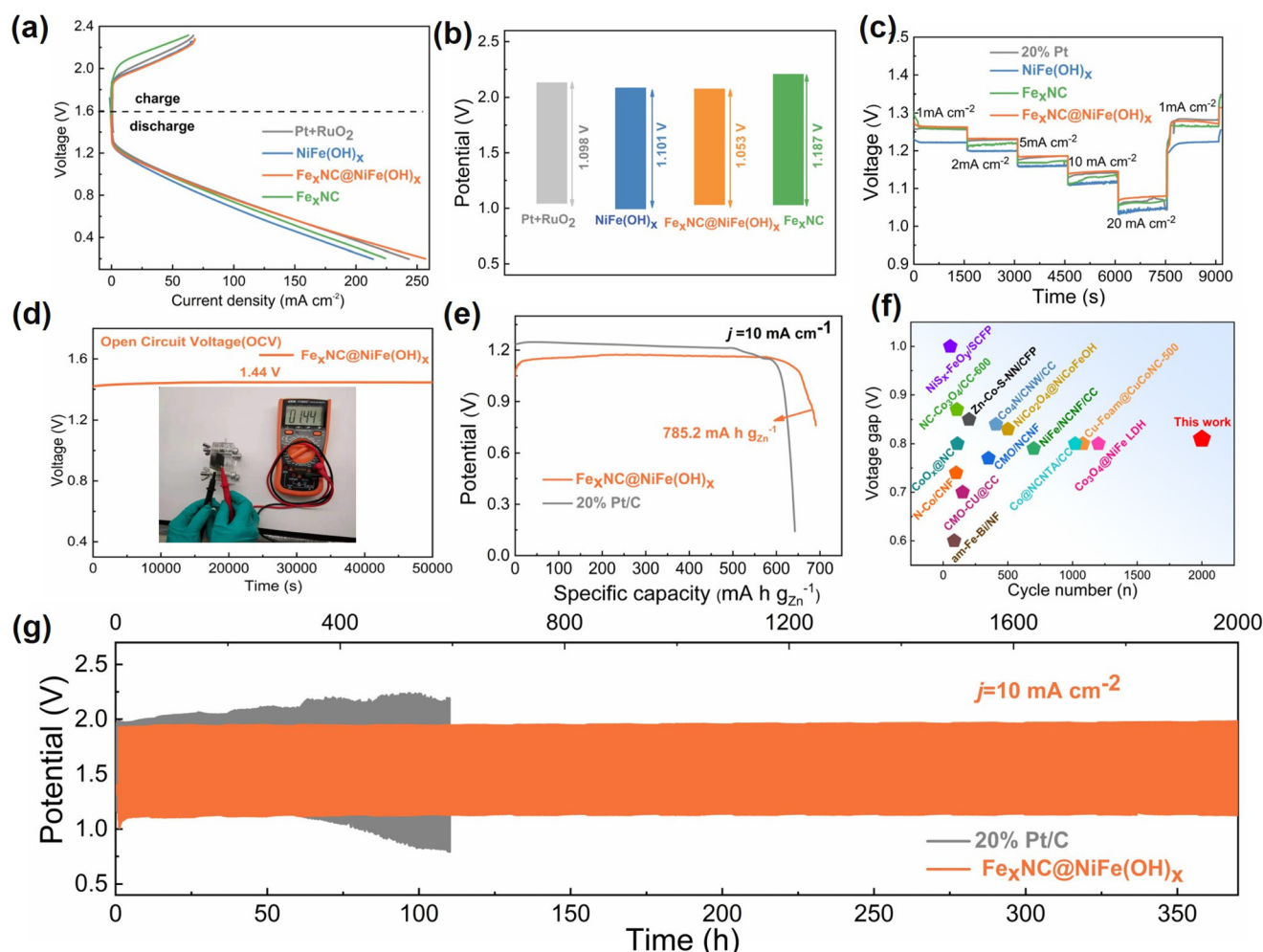
Fig. 4 (a) The charge/discharge polarization curves. (b) Voltage gaps at the current density of 40 \text{ mA cm}^{-2} . (c) Galvanostatic discharge of Pt/C-ZAB, \text{Fe}_x\text{NC} -ZAB, \text{NiFe}(\text{OH})_x -ZAB, and \text{Fe}_x\text{NC}@ \text{NiFe}(\text{OH})_x -ZAB under different current densities. (d) Open circuit potential, inset: optical image. (e) The specific capacity curves run at 10 \text{ mA cm}^{-2} . (f) Performance comparison of ZABs using self-supported bifunctional electrodes operating at 10 \text{ mA cm}^{-2} . (g) The discharge/charge cycle curves of Pt/C-ZAB and \text{Fe}_x\text{NC}@ \text{NiFe}(\text{OH})_x -ZAB at 10 \text{ mA cm}^{-2} .
