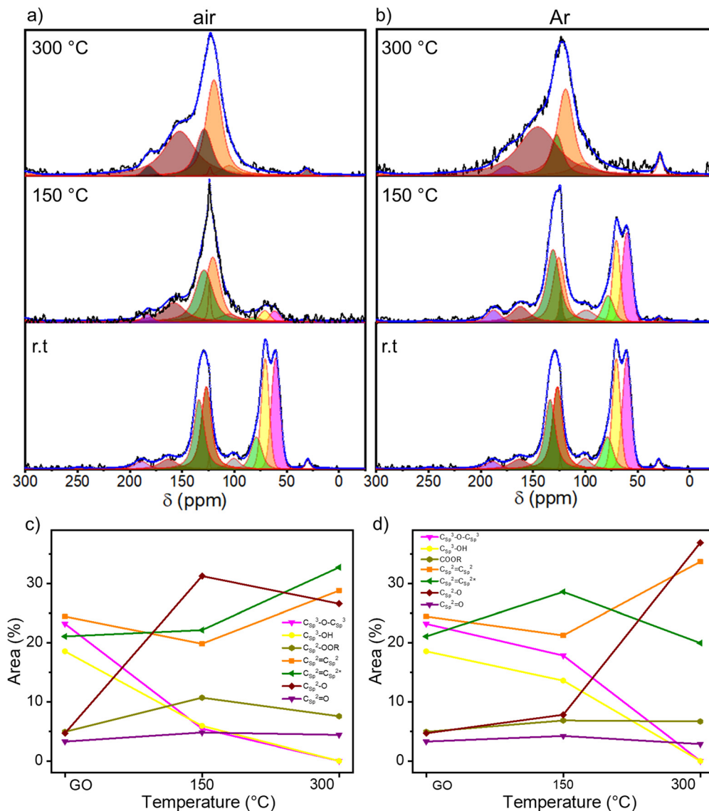
Fig. 3 Solid-state MAS-NMR \text{C } 1\text{s} spectra of thermally rGO under (a) air and (b) argon; temperature dependence of the relative contribution of NMR spectral components estimated by dividing the area under each component by the whole peak area for (c) air and (d) argon.
