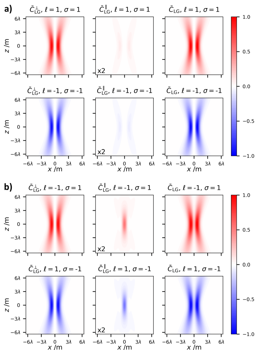
Fig. 6 Diffractive properties of the (left) transverse, \bar{C}_{LG}^{\perp} , (centre) longitudinal, \bar{C}_{LG}^{\parallel} , and (right) combined, \bar{C}_{LG} , field contributions to the optical chirality densities of circularly polarised \sigma = \pm 1 LG ( \ell = \pm 1 , p = 0 ) beams, normalised to the total, \bar{C}_{LG} . (a) Parallel SAM and OAM, \text{sgn } \ell = \text{sgn } \sigma . (b) Anti-parallel SAM and OAM \text{sgn } \ell \neq \text{sgn } \sigma . In all plots w_0 = \lambda .
