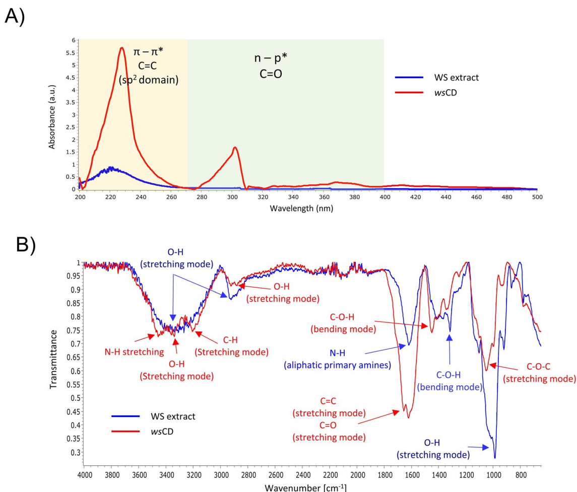
Fig. 2 Chemical structure and surface functional group analysis. (A) Chemical structure analysis of WS extract and \omega\text{CDs} using UV absorption spectroscopy; (B) surface functional group analysis of WS extract (blue) and \omega\text{CDs} (red) using Fourier transform infrared spectroscopy.
