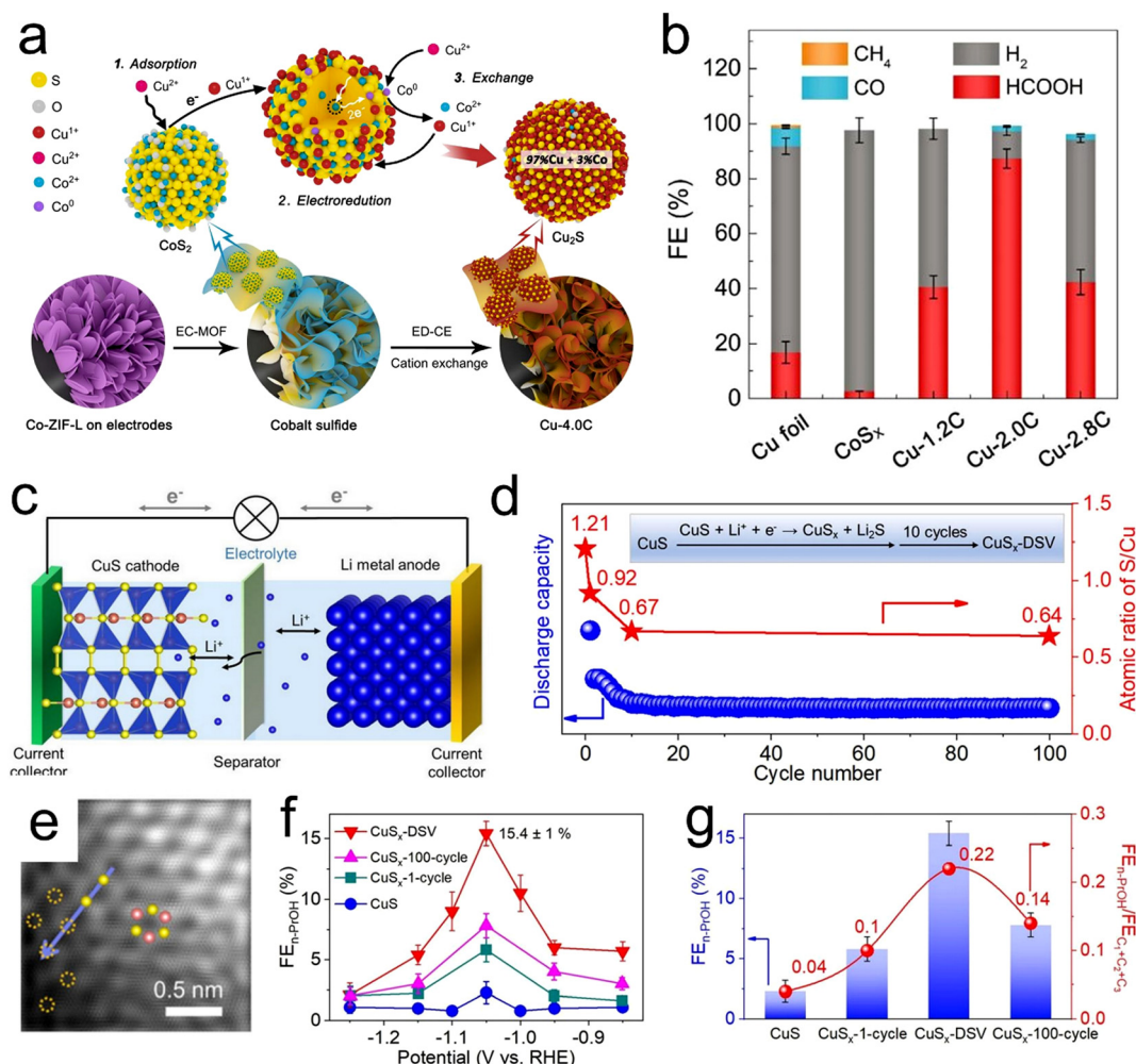
Fig. 7 (a) Diagram of the experimental paths and mechanisms for electrochemically-driven cation exchange, (b) FE values for CO 2 RR products using Cu foil, \text{CoS}_x , Cu-1.2C, Cu-2.0C and Cu-2.8C at -0.9 V (vs. RHE). (c) Diagram of a lithium-ion battery assembled with CuS (cathode) and Li metal (anode), (d) discharge capacities of CuS (blue dots) and the S/Cu atomic ratios (red stars) with respect to the cycle number at a constant current of 0.044 \text{ mA cm}^{-2} in the voltage range of 0.01\text{--}3 V. Sulfur atoms in the CuS lattice were selectively removed to form \text{Li}_2\text{S} , resulting in \text{CuS}_x -DSV. (e) HAADF-STEM image of \text{CuS}_x -DSV and (f and g) FE and \text{FE}_{n\text{-PrOH}} values together with \text{FE}_{n\text{-PrOH}}/\text{FE}_{\text{C}_1+\text{C}_2+\text{C}_3} ratios for n -propanol on four catalysts (CuS, \text{CuS}_x -1-cycle, \text{CuS}_x -DSV and \text{CuS}_x -100-cycle) at different applied potentials. Reproduction with permission from ref. 121, Copyright 2020, Wiley-VCH and Reproduction with permission from ref. 63, Copyright 2021, Springer Nature.
