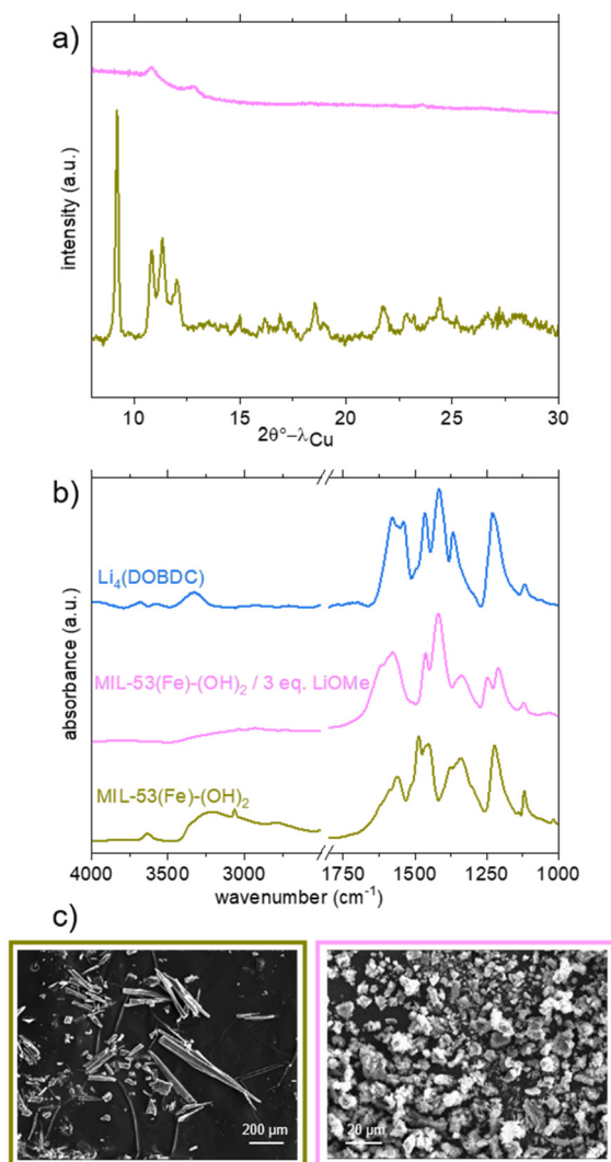
Fig. 5 Characterisation of \text{MIL-53(Fe)-(OH)}_2 and its lithiated product from LiOMe in MeOH/THF. a) PXRD patterns ( \lambda = 1.5406\text{ }\text{\AA} ); b) IR spectra; c) SEM pictures. Data related to dry \text{MIL-53(Fe)-(OH)}_2 , \text{Li}_4(\text{DOBDC}) and the lithiation product are shown in khaki, blue and pink, respectively.
