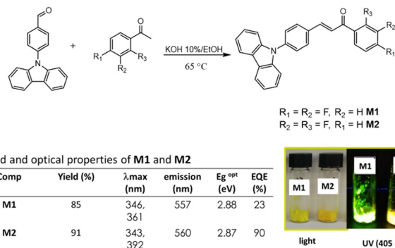
Fig. 1 Synthetic route of chalcones M1 and M2 , and solid-state absorption and emission.
