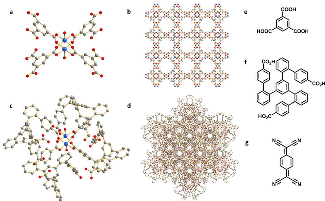
Fig. 1 Views of (a) the [Cu_2(OOCR)_4] paddlewheel in HKUST-1; (b) structure of HKUST-1; (c) the [Cu_2(OOCR)_4] paddlewheel in CuMOP; (d) structure of CuMOP; (e) benzene-1,3,5-tricarboxylic acid used in HKUST-1; (f) ligand used in CuMOP; (g) TCNQ. Cu: blue; O: red; C: grey; hydrogen atoms are omitted for clarity.
