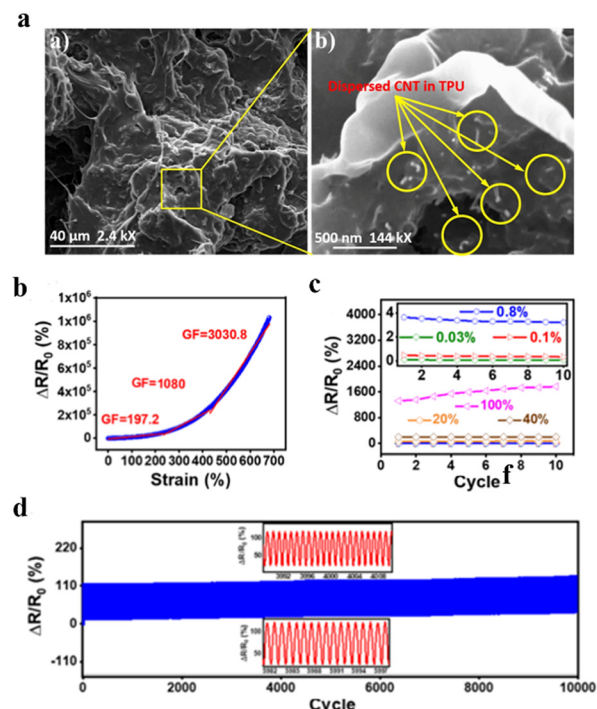
Fig. 12 (a) SEM images of TPU/MWCNT/AgNPs. Reproduced with permission from ref. 180. Copyright 2019, Wiley-VCH. (b) \Delta R/R_0 of CPUF vs strain. (c) Maximum values of CPUF at the strain of 0.03% to 100%. (d) Long-term stability during 10 000 cycles. Reproduced with permission from ref. 182. Copyright 2022, the American Chemistry Society.
