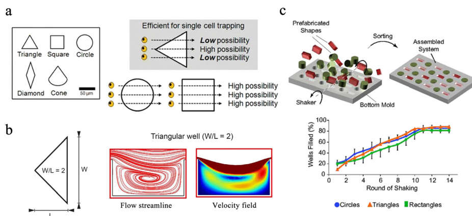
Fig. 2 Different designs of microwell chips for single-cell analysis. (a) The equilateral triangle has been proven to be an ideal well shape. Scale bar: 50 \mu\text{m} . Reproduced with permission. 32 Copyright 2009, Springer Nature Publishing. (b) Triangular microwell with W/L = 2 has the best trapping capability because of the enhanced recirculation vortex. Reproduced with permission. 39 Copyright 2019, Springer Nature Publishing. (c) Extensive compositional and geometric tunability of shape-coded microwell patterns. Reproduced with permission. 38 Copyright 2013, National Academy of Sciences.
