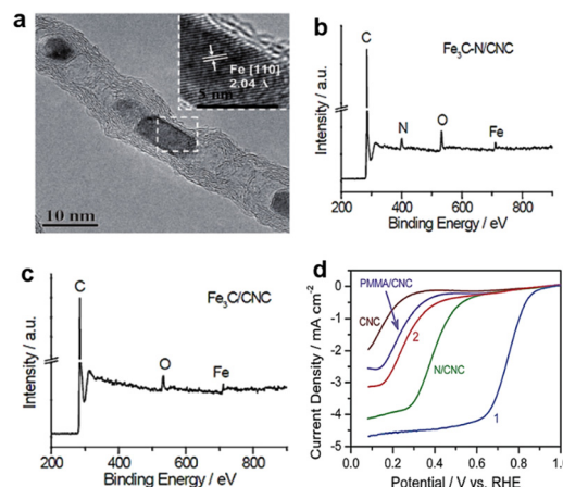
Fig. 4 (a) High resolution transmission electron microscopy (HRTEM) image of \text{Fe}_3\text{C}-\text{N}/\text{CNC} with the inset showing the [110] crystal plane of \text{Fe} . 25 XPS spectra of (b) \text{Fe}_3\text{C}-\text{N}/\text{CNC} and (c) \text{Fe}_3\text{C}/\text{CNC} . 29 (d) ORR performance of \text{Fe}_3\text{C}-\text{N}/\text{CNC} (curve 1) and \text{Fe}_3\text{C}/\text{CNC} (curve 2). 29
